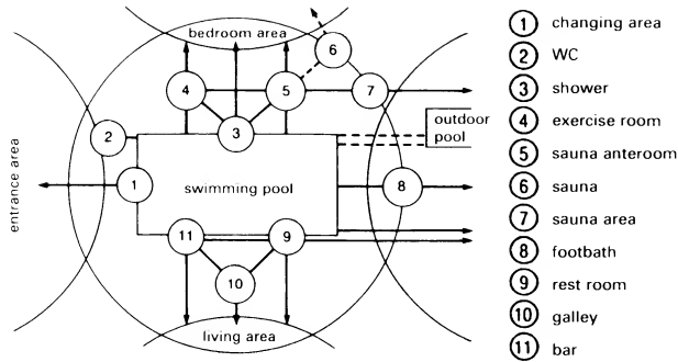
1 Layout of an integrated swimming pool in a single family house
